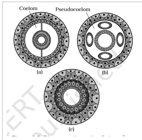
Fig. 4.3 - Diagrammatic sectional view of : (a) Coelomate (b) Pseudocoelomate (c) Acoelomate. Labels: Coelom and Pseudocoelom.
